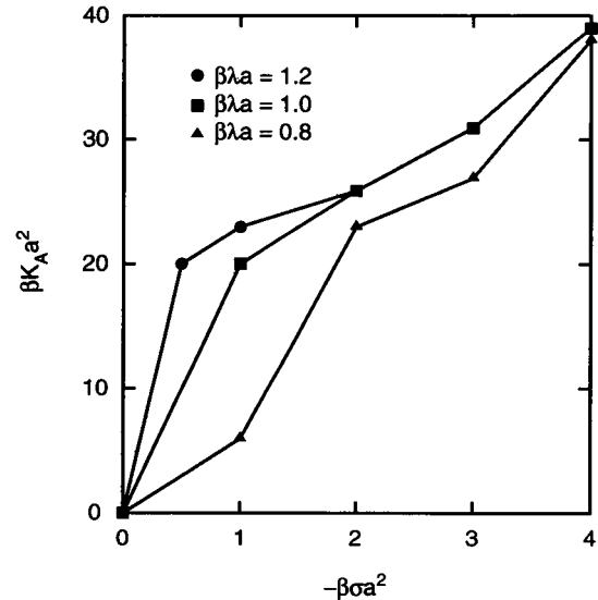
FIGURE 6 Dimensionless area compression modulus \beta K_A a^2 as a function of applied stress for three values of the edge tension \beta\lambda a = 0.8, 1.0 , and 1.2 . The moduli are determined from a system with N = 196 vertices.
