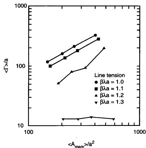
FIGURE 4 Average hole perimeter \langle \Gamma \rangle / a plotted against average membrane area \langle A_{\text{mem}} \rangle / a^2 for zero stress and edge tensions \beta \lambda a = 1.0 , 1.1, 1.2, and 1.3. Each data point is determined at a fixed value of N : 144, 196, 256, and 400.
