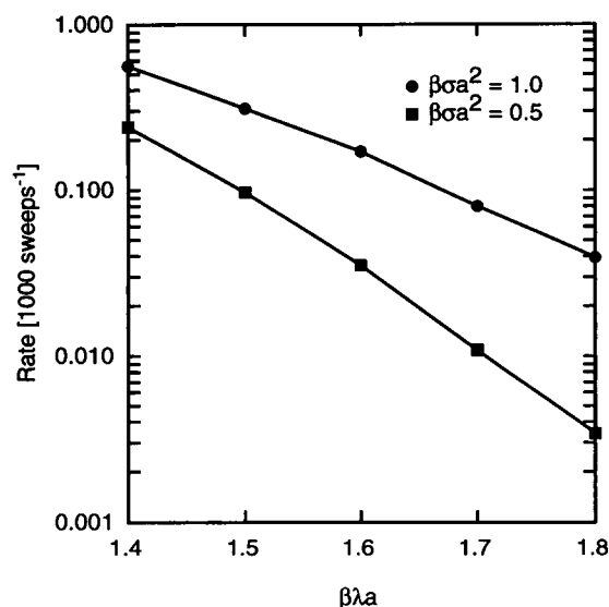
FIGURE 8 Rupture rates as a function of edge tension at two values of the applied surface stress: \beta\sigma a^2 = 0.5 and 1.0 . The rate shown here is \langle \tau \rangle^{-1} ; see text after Eq. 9 for discussion.
